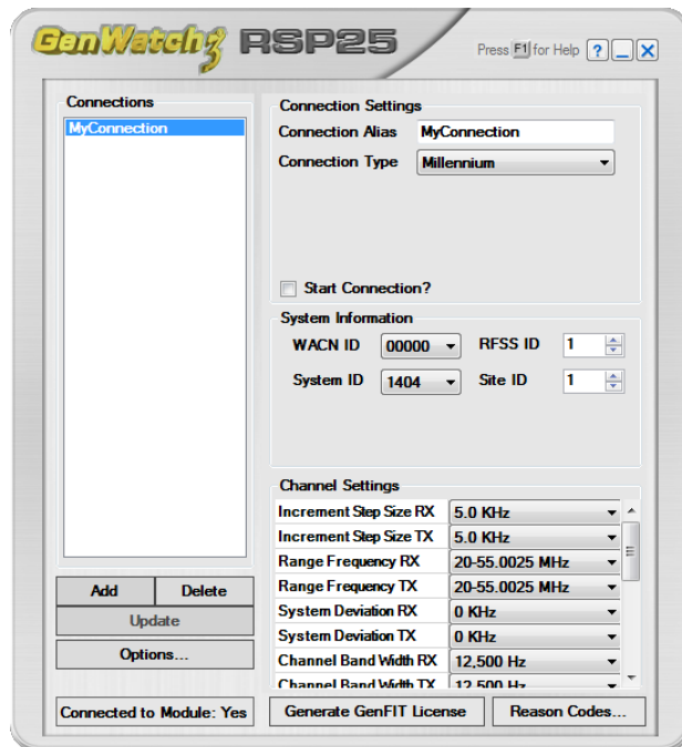
Figure 3.1 – GW_RSP25 GUI
